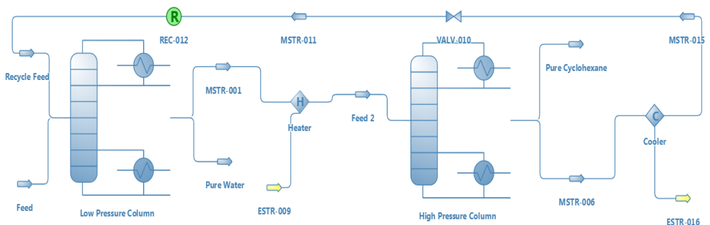
Pressure Swing Distillation of Water-Cyclohexane Mixture
